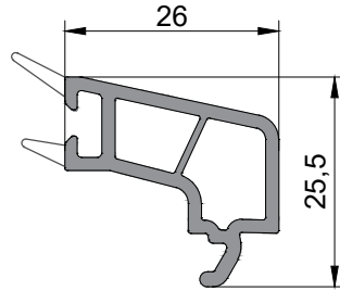
Glazing bead for sliding (Single)
