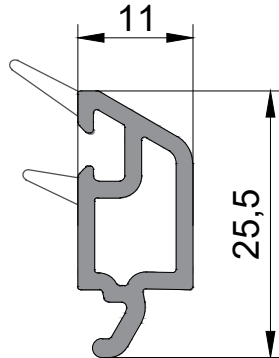
Glazing bead for casemet (another option)
