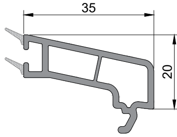
Glazing bead for casemet (Single)
