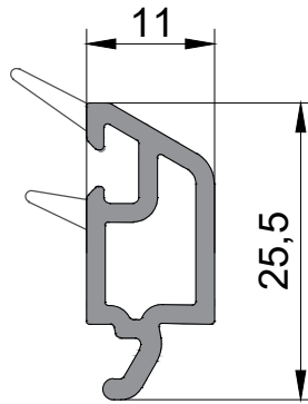
Glazing bead for sliding (Double)
