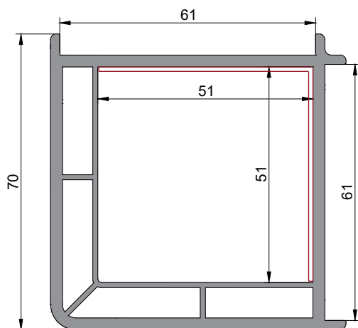
90 Degree corner profile upvc
