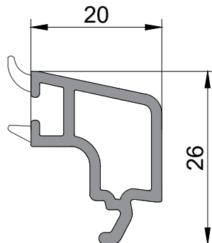
Glazing bead for sliding (another option)
