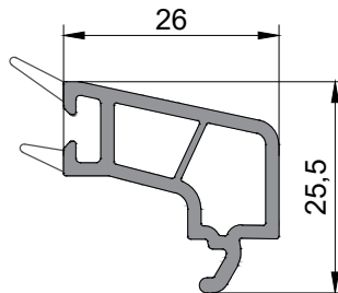
Glazing bead for casemet (another option)
