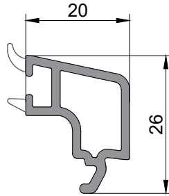
Glazing bead for casemet (Double)
