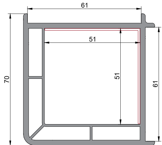
90 Degree corner profile upvc
