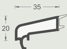
EMA4279 Single glazing bead 20 pieces/ package
