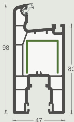
EMA1221 Sliding frame profile 6 pieces/ package
