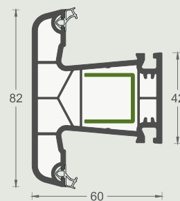
EMA4275 Mullion profile 6 pieces/ package
