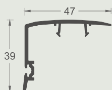
EMA5014 Interlock profile 10 pieces/ package
