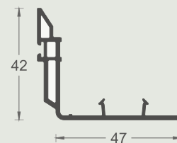
EMA1225 Window interlock profile 10 pieces/ package
