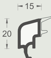
EMA4278 Double glazing bead 25 pieces/ package
