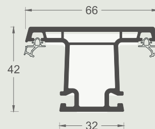
EMA5017 Mullion profile 6 pieces/ package
