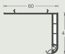
EMA4282 Frame sill profile 10 pieces/ package
