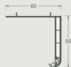
EMA6710 Frame sill profile 10 pieces/ package
