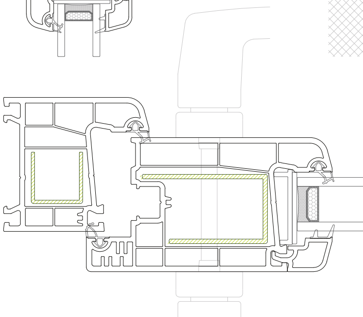
Section C Horizontal section of door sash and frame connection
