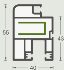
EMA1223 Mosquito sash profile 15 pieces/ package
