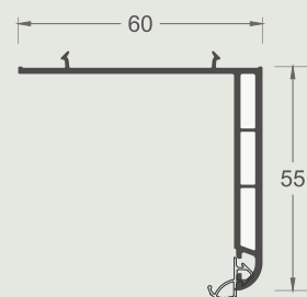
EMA6710 Frame sill profile 10 pieces/ package
