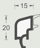
EMA4278 Double glazing bead 25 pieces/ package
