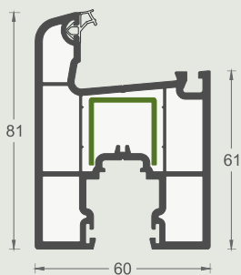
EMA4283 Sliding sash profile 6 pieces/ package
