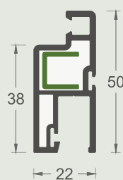
EMA5015 Mosquito sash profile 15 pieces/ package
