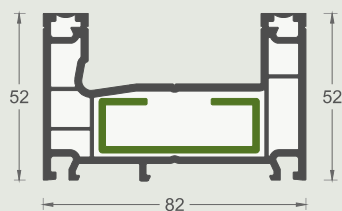
EMA4280 Sliding frame profile 4 pieces/ package
