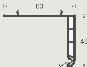
EMA4282 Frame sill profile 10 pieces/ package
