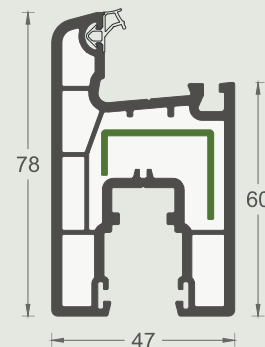
EMA1220 Sliding window sash profile 6 pieces/ package
