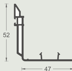
EMA1224 Door interlock profile 10 pieces/ package
