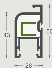
EMA4285 Mosquito sash profile 15 pieces/ package
