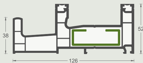
EMA4281 Fixed sliding frame profile 6 pieces/ package
